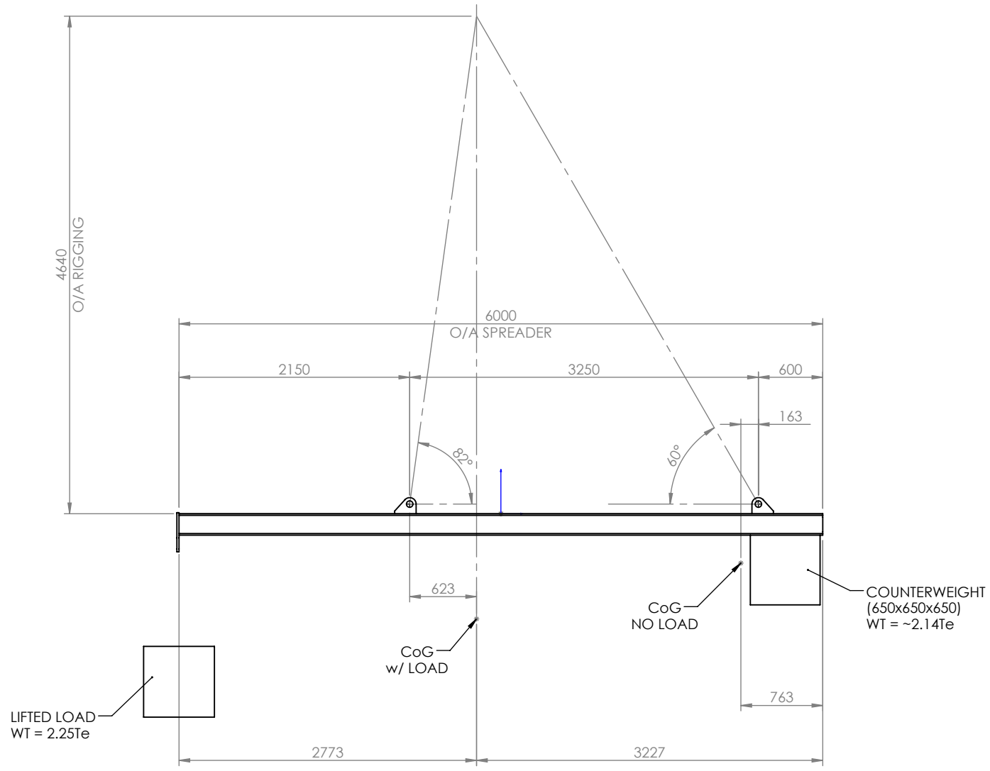
ELEVATION - 3Te SPREADER
